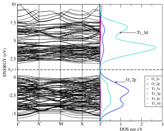
FIG. 10: BS and PDOS of 5L-TiO 2 rutile clean (110) surface
